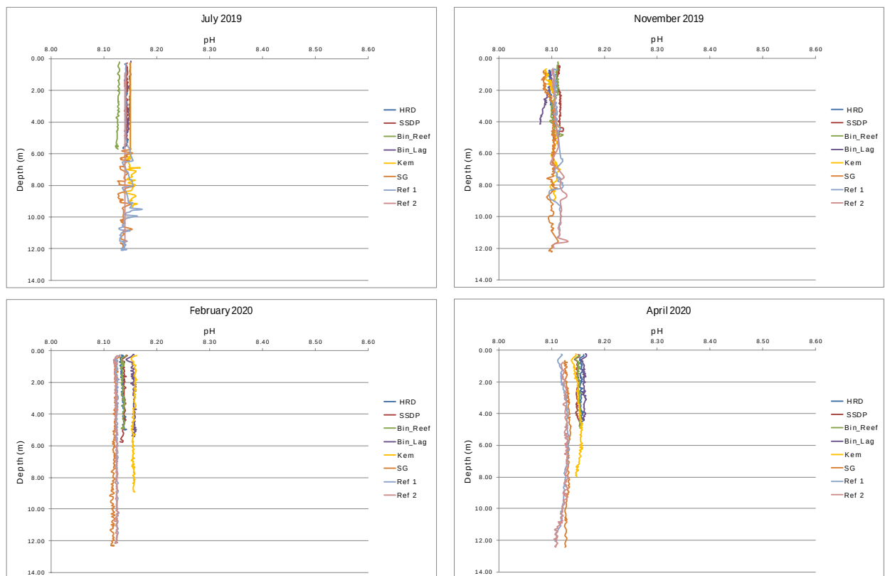
Figure 6: pH at each of the sites during July 2019 (top left), November 2019 (top right), February 2020 (bottom left) and April 2020 (bottom right)
