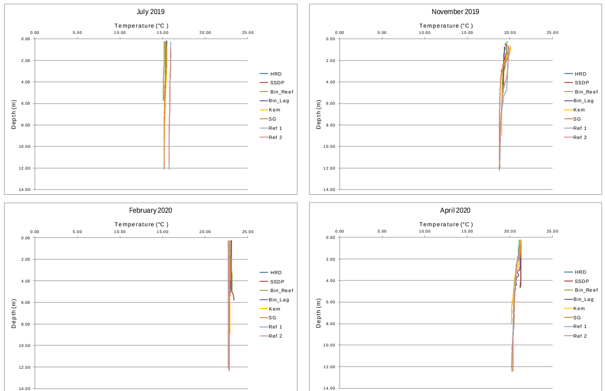
Figure 5: Temperature at each of the sites during July 2019 (top left), November 2019 (top right), February 2020 (bottom left) and April 2020 (bottom right)
