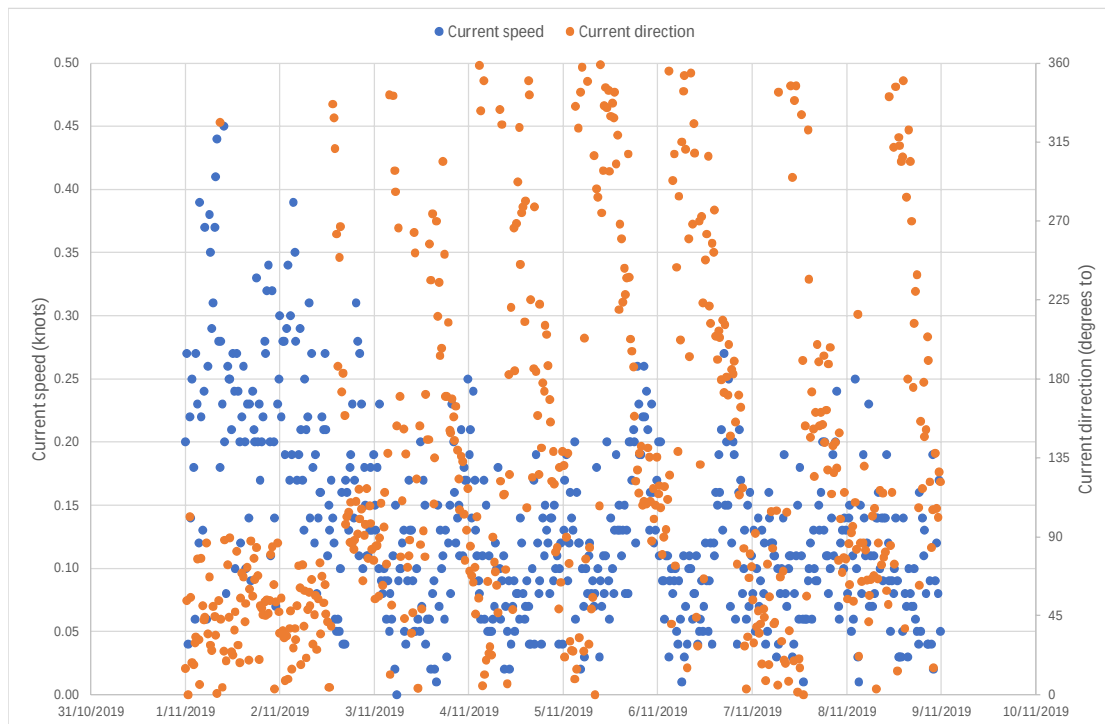
Current speed and direction 1-8 November 2019
