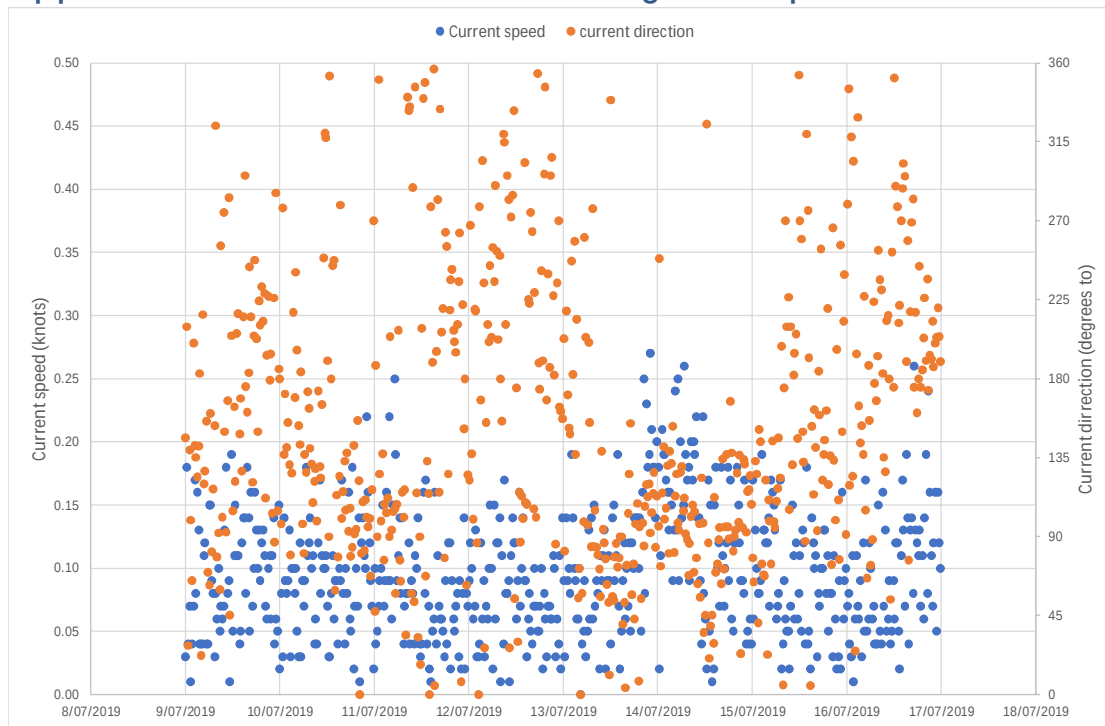
Current speed and direction 9-17 July 2019
