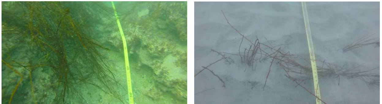
Figure 15: The 24 m mark on the transect at Bin_Lag in July 2020 (left) showing reef and Polysiphonia sertularioides growing on top of the reef and in November 2020 (right) with the reef completely buried and only the tops of P. sertularioides visible.
