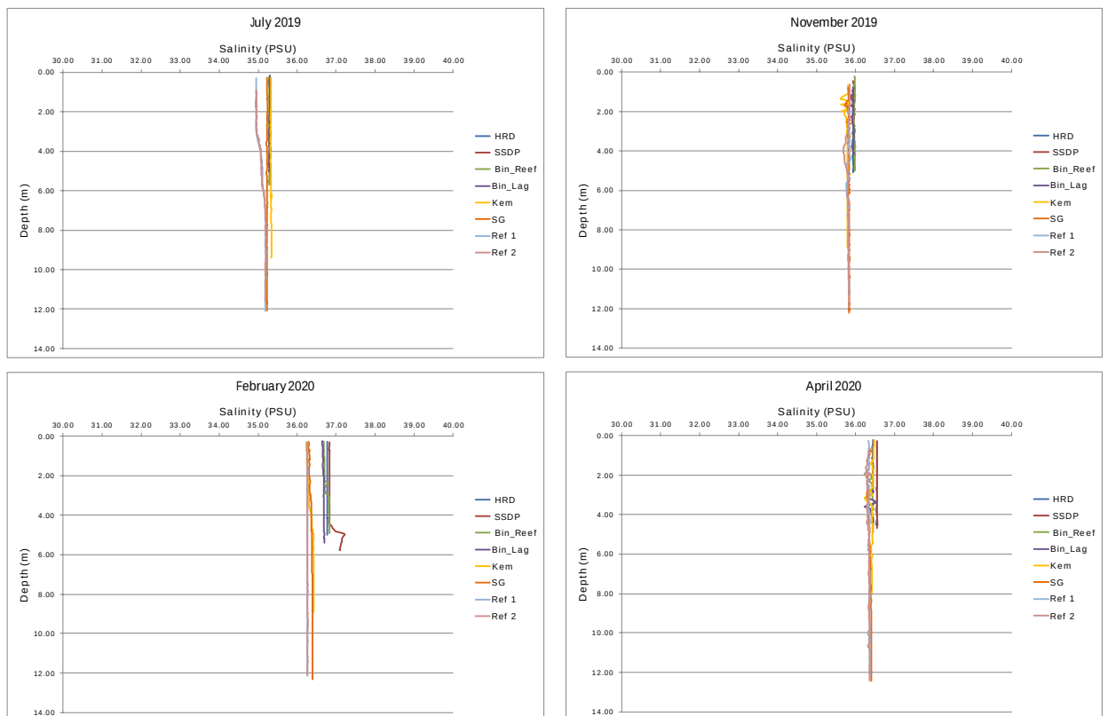
Figure 4: Salinity at each of the sites during July 2019 (top left), November 2019 (top right), February 2020 (bottom left) and April 2020 (bottom right)
