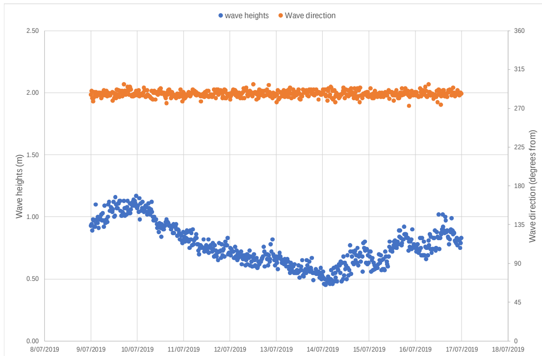
Significant wave heights and direction 9-17 July 2019
