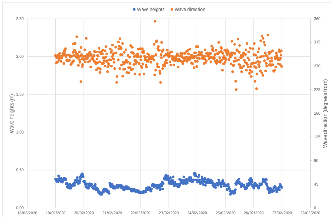
Significant wave heights and direction 19-27 February 2020
