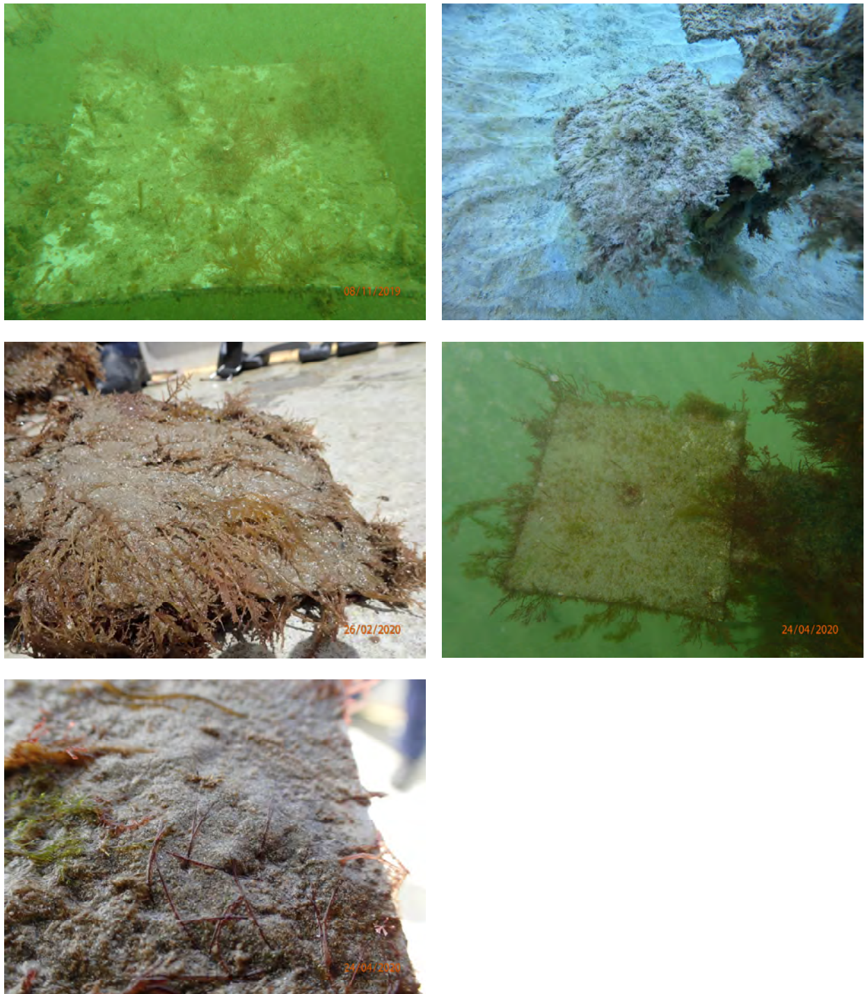
Figure 12: Settlement plates at site Bin_Lag at the end of the July-November 2019 deployment (top left), November 2019 – February 2020 (top right and middle left) and February-April 2020 (middle right). The bottom photo shows a close up of the algae trapping the sediment to the plate.
