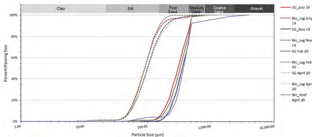
Figure 9: Particle size distribution of the sediments of sites SG and Bin_Lag over the four sampling occasions and Bin_Reef in April 2020 as a line graph.
